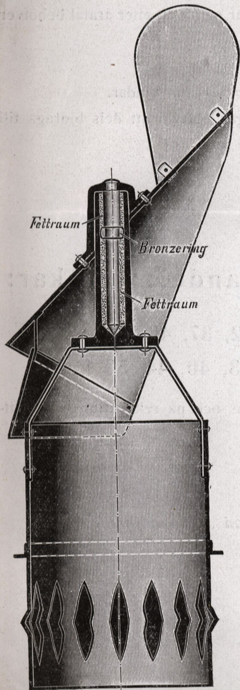
Genomskärning.
