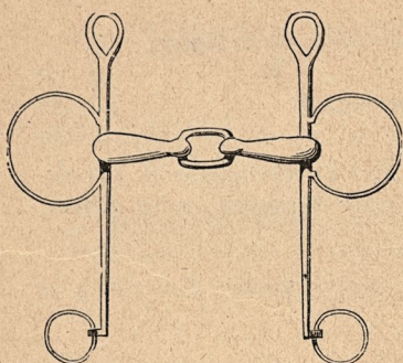
50. Boltensterns Pelham.
