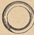
112. Gummi-strykring.
