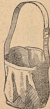
145. To mister.
