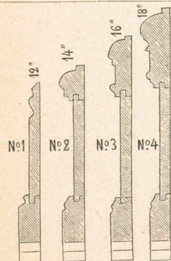
SOCKEL-PANEL.
