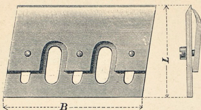
Planboxjern.
