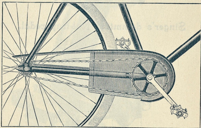
The Singer Semi-Gear-Case.
