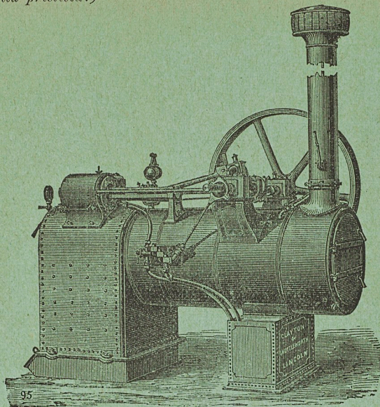
Clayton & Shuttleworths halftransportabel Lokomobil.
