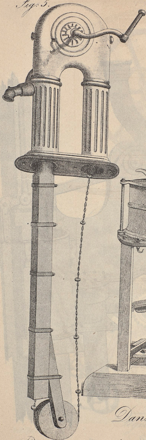
Paternosterpump.
