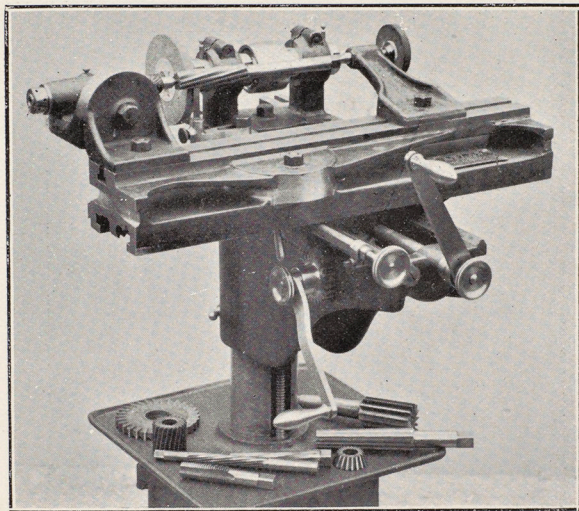
Sharpening reamers and cutters.
