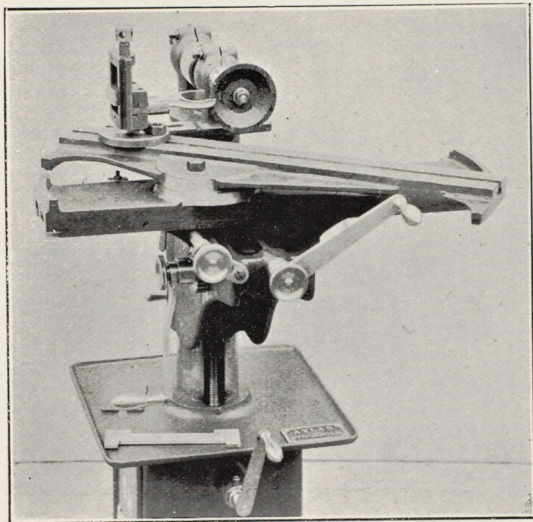
Grinding gauges.
